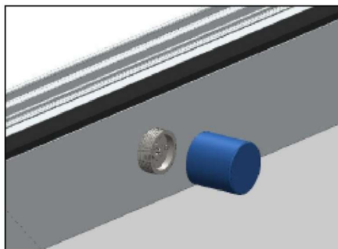
7. Screw the outer sleeve
